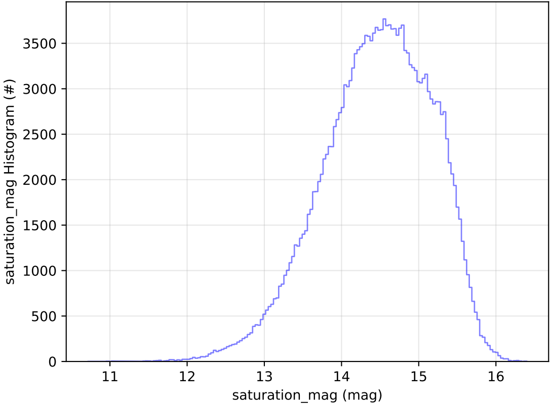
too_elab_r32_d3_griz_v3.4_10yrs All sky g band: saturation_mag Histogram
