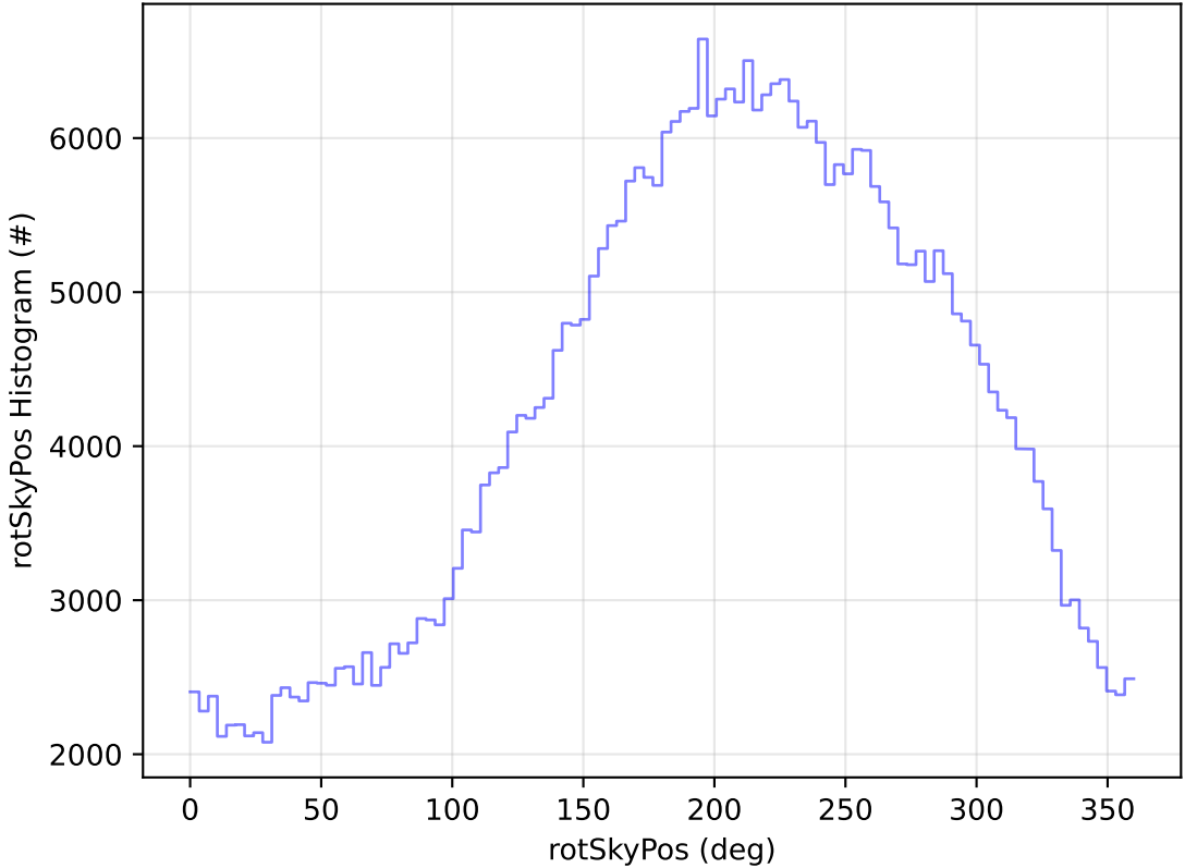
too_elab_r32_d3_griz_v3.4_10yrs WFD z band: rotSkyPos Histogram
