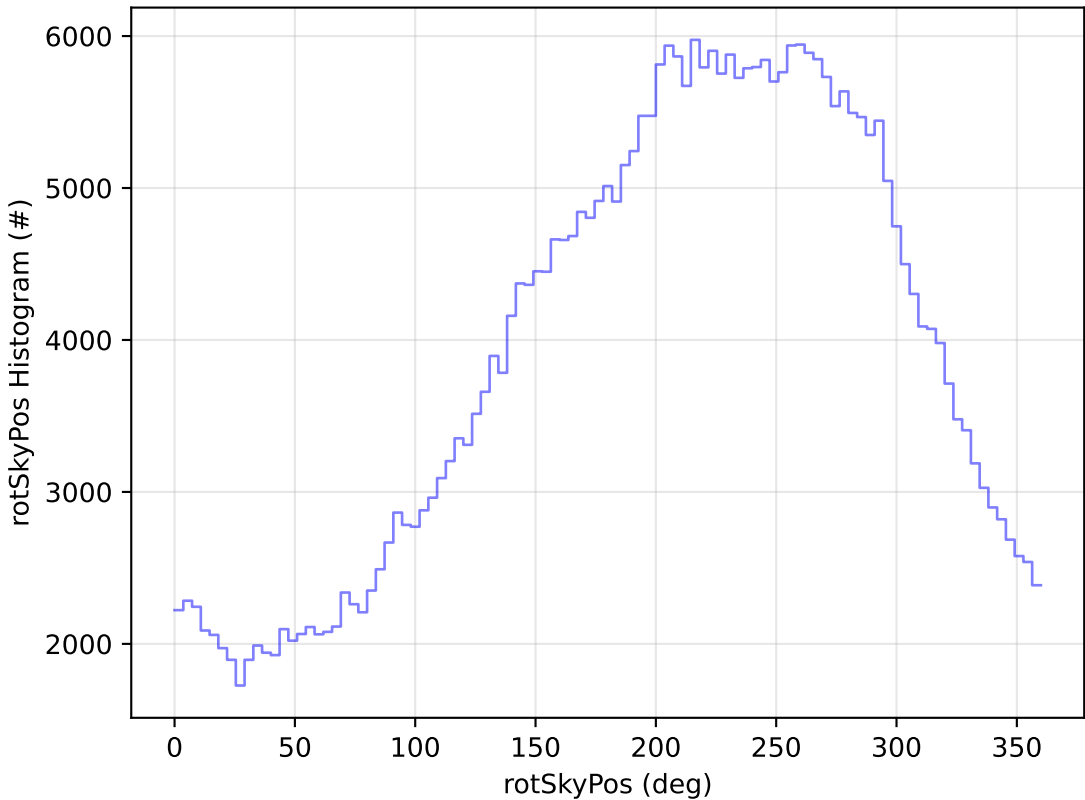
too_elab_r32_d3_griz_v3.4_10yrs WFD y band: rotSkyPos Histogram
