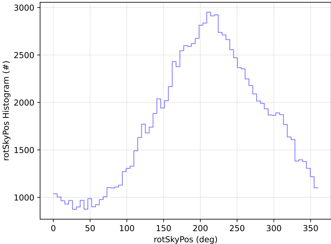
too_elab_r32_d3_griz_v3.4_10yrs WFD u band: rotSkyPos Histogram
