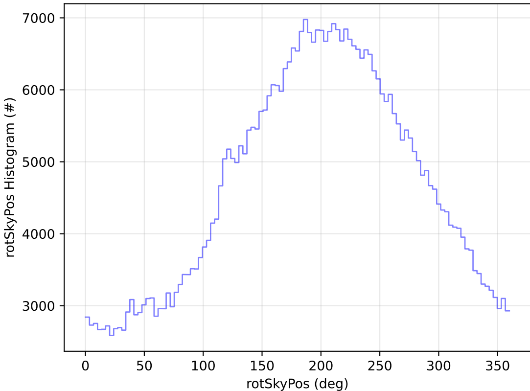
too_elab_r32_d3_griz_v3.4_10yrs WFD r band: rotSkyPos Histogram
