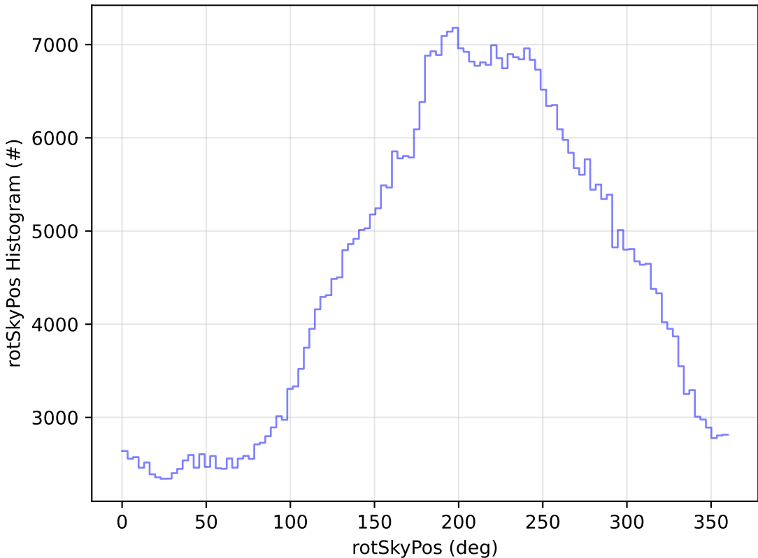
too_elab_r32_d3_griz_v3.4_10yrs WFD i band: rotSkyPos Histogram
