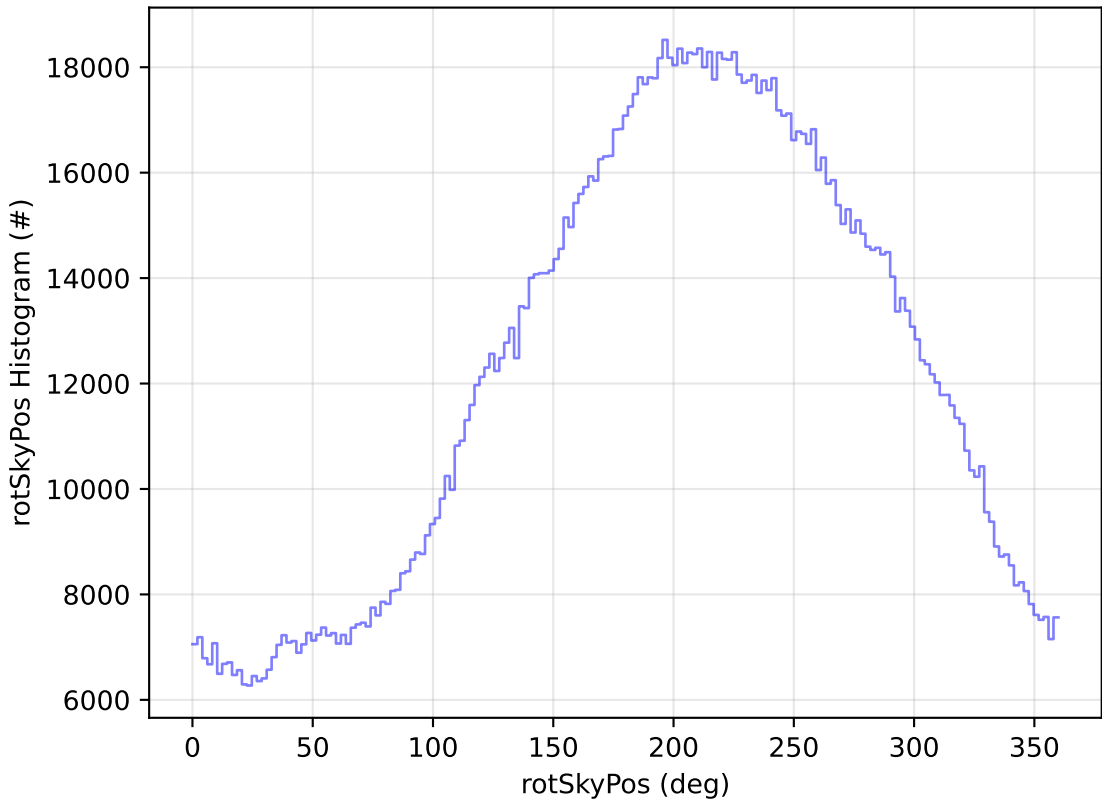
too_elab_r32_d3_griz_v3.4_10yrs WFD all bands: rotSkyPos Histogram
