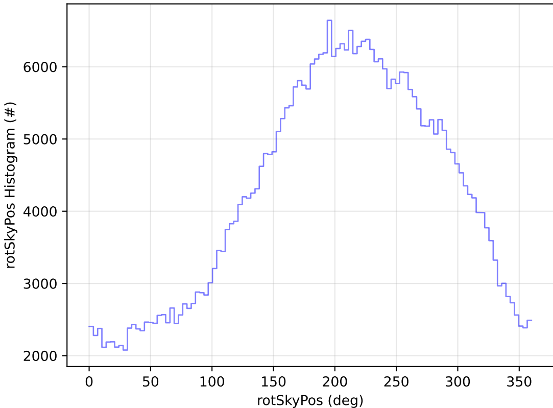
too_elab_r32_d3_griz_v3.4_10yrs All sky z band: rotSkyPos Histogram
