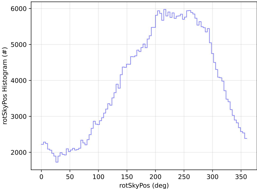
too_elab_r32_d3_griz_v3.4_10yrs All sky y band: rotSkyPos Histogram
