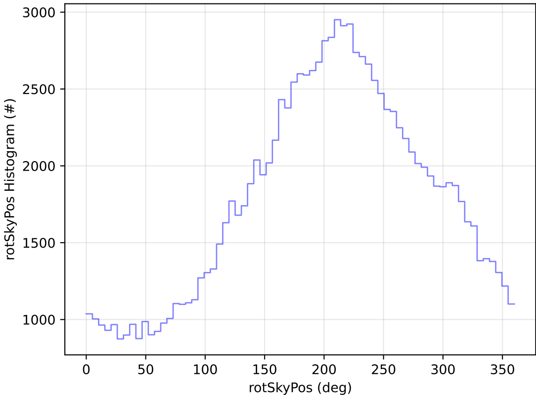
too_elab_r32_d3_griz_v3.4_10yrs All sky u band: rotSkyPos Histogram
