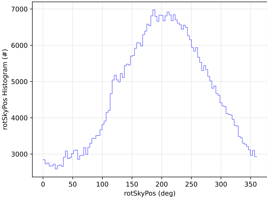
too_elab_r32_d3_griz_v3.4_10yrs All sky r band: rotSkyPos Histogram
