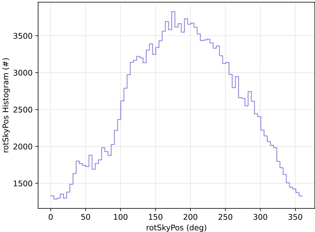
too_elab_r32_d3_griz_v3.4_10yrs All sky g band: rotSkyPos Histogram
