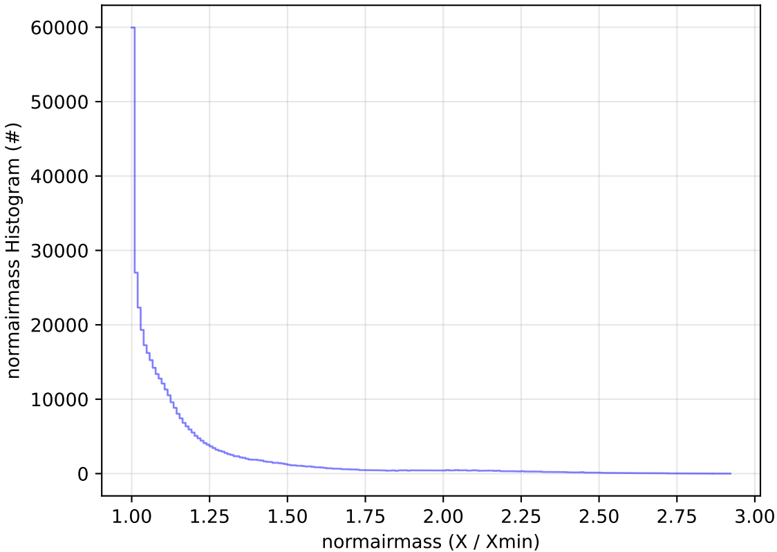
too_elab_r32_d3_griz_v3.4_10yrs WFD z band: normairmass Histogram
