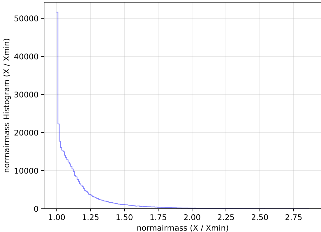
too_elab_r32_d3_griz_v3.4_10yrs WFD y band: normairmass Histogram
