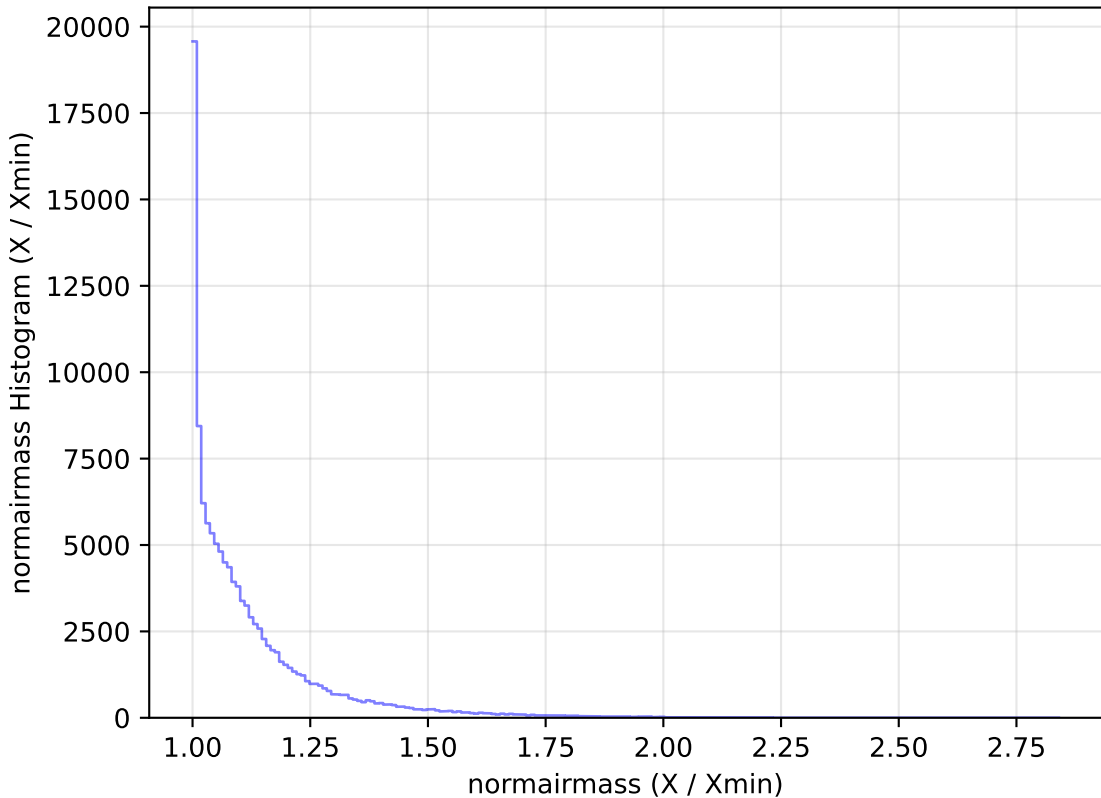
too_elab_r32_d3_griz_v3.4_10yrs WFD u band: normairmass Histogram
