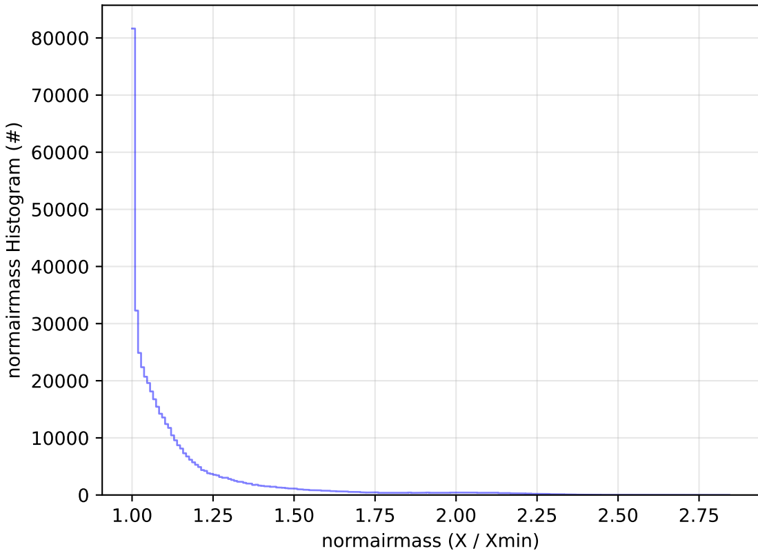
too_elab_r32_d3_griz_v3.4_10yrs WFD r band: normairmass Histogram
