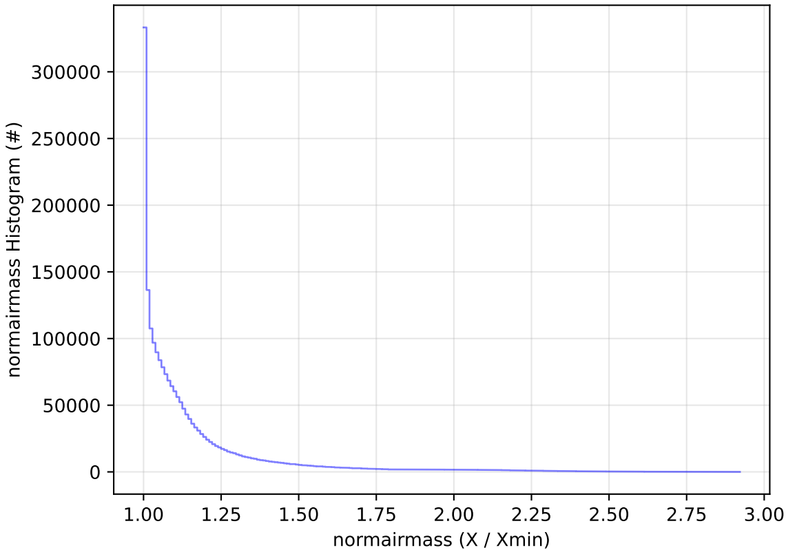
too_elab_r32_d3_griz_v3.4_10yrs WFD all bands: normairmass Histogram
