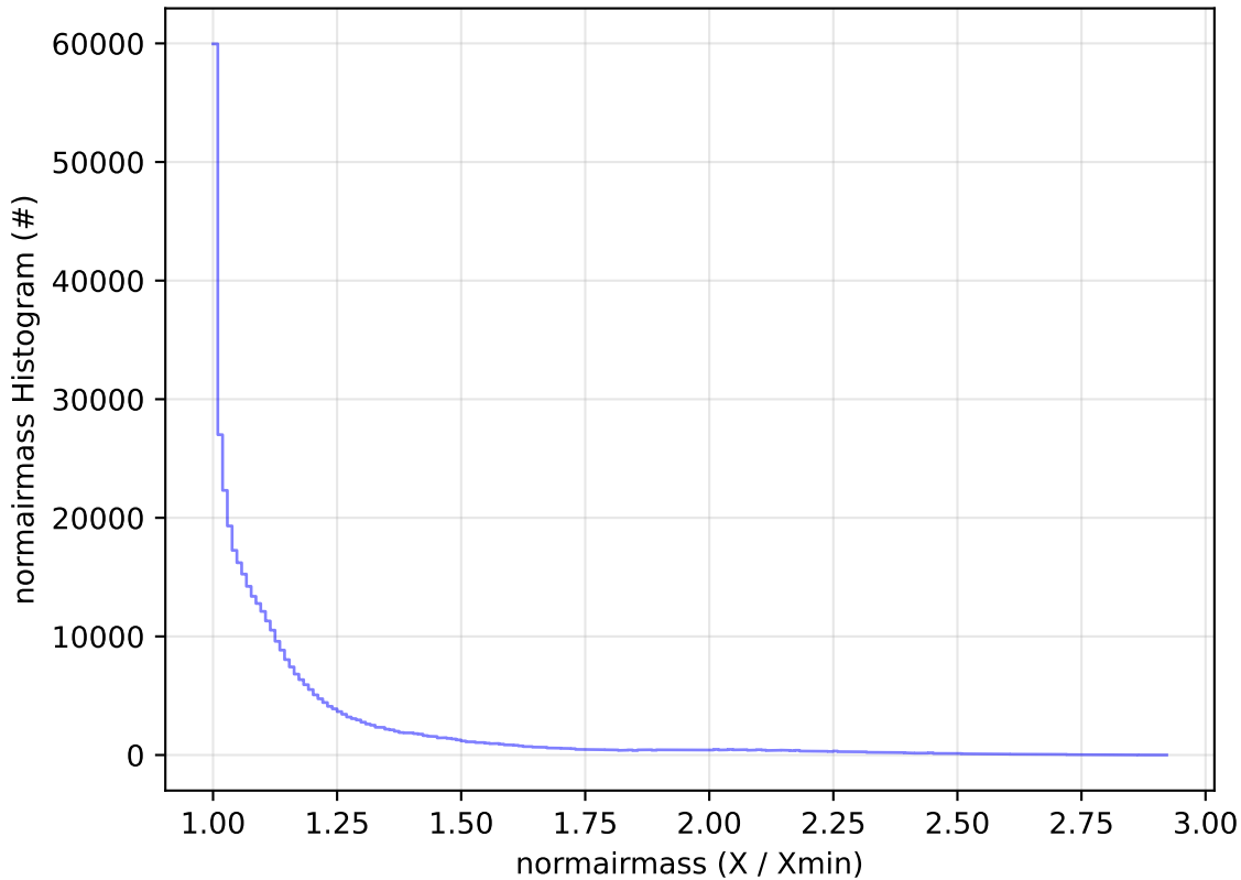
too_elab_r32_d3_griz_v3.4_10yrs All sky z band: normairmass Histogram
