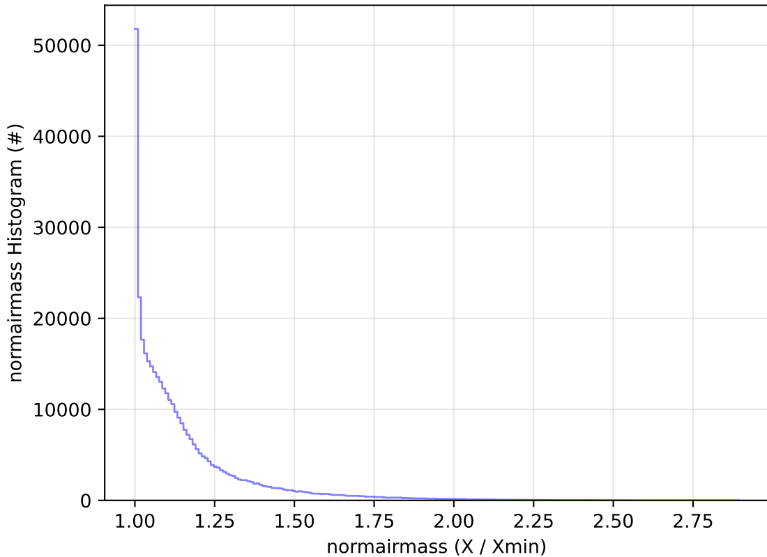
too_elab_r32_d3_griz_v3.4_10yrs All sky y band: normairmass Histogram
