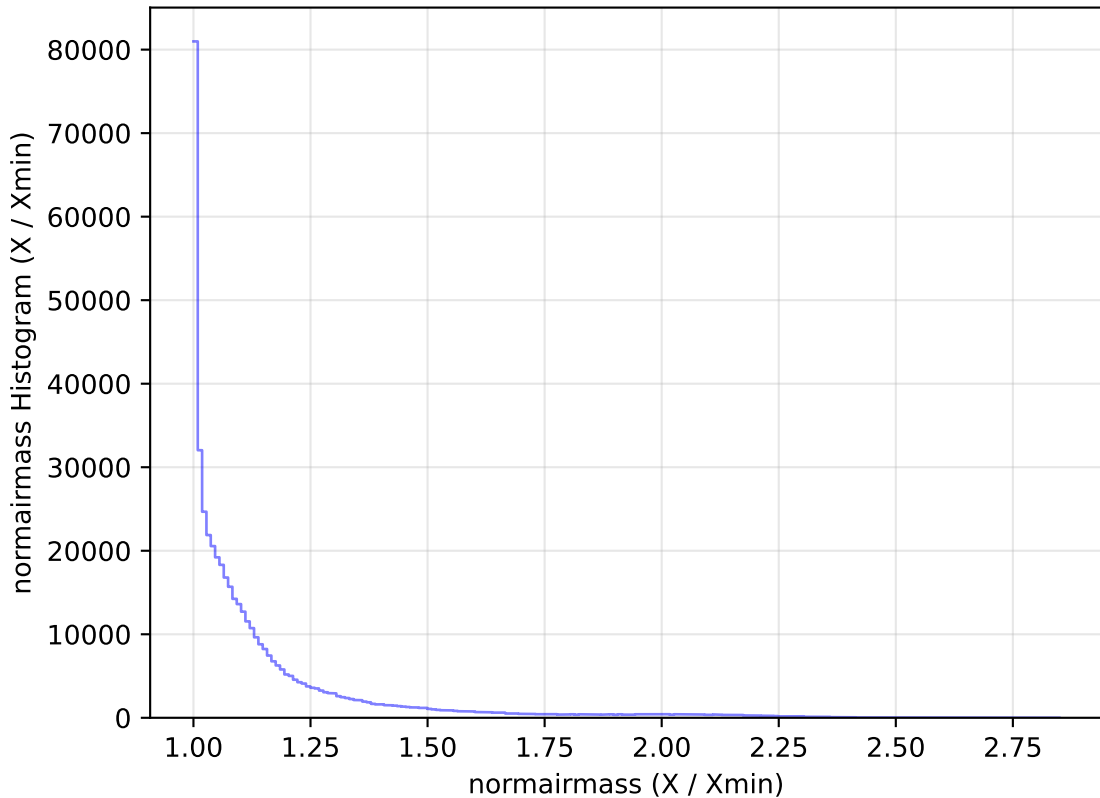
too_elab_r32_d3_griz_v3.4_10yrs All sky r band: normairmass Histogram
