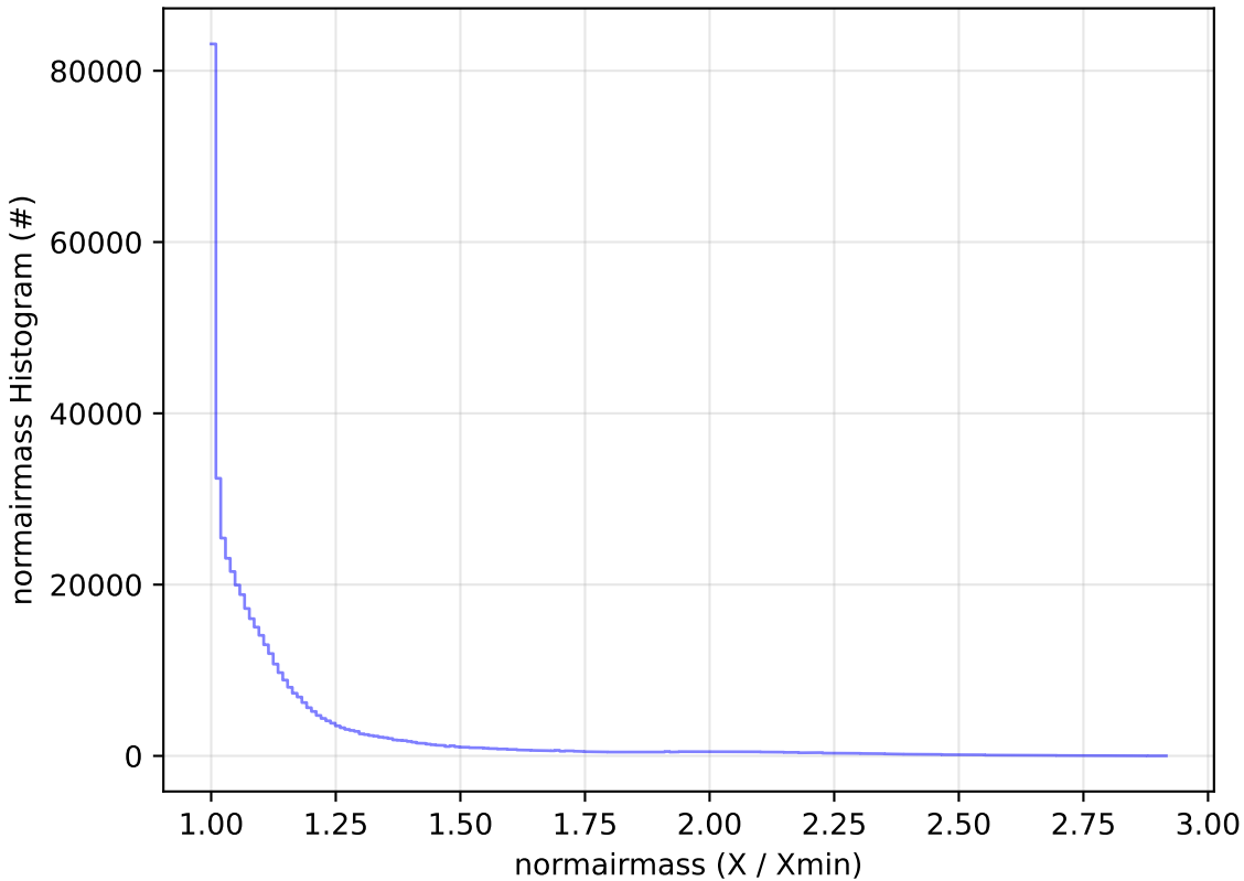
too_elab_r32_d3_griz_v3.4_10yrs All sky i band: normairmass Histogram
