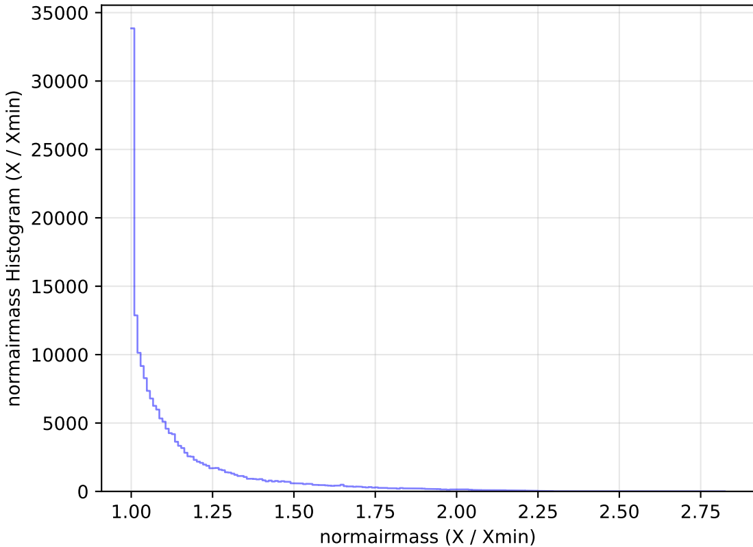
too_elab_r32_d3_griz_v3.4_10yrs All sky g band: normairmass Histogram
