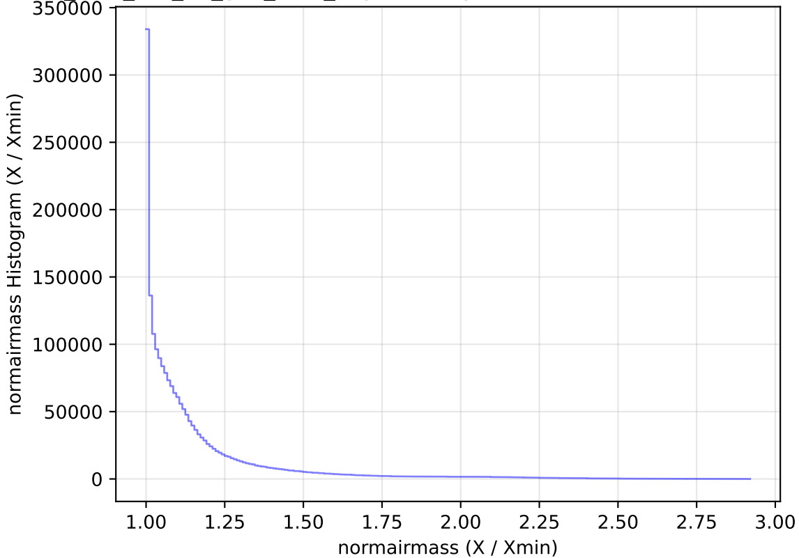
too_elab_r32_d3_griz_v3.4_10yrs All sky all bands: normairmass Histogram
