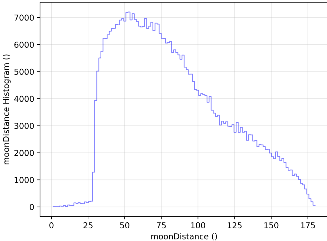
too_elab_r32_d3_griz_v3.4_10yrs WFD z band: moonDistance Histogram
