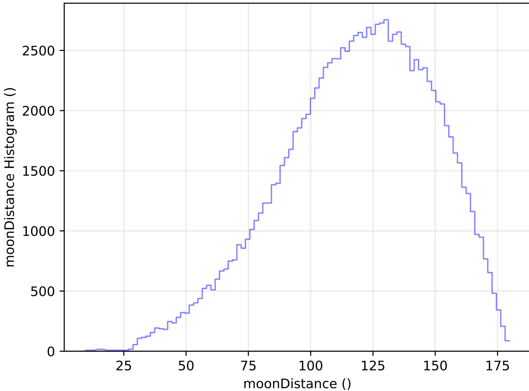
too_elab_r32_d3_griz_v3.4_10yrs WFD u band: moonDistance Histogram
