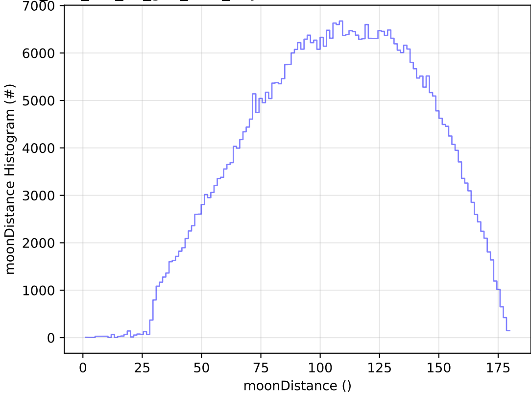
too_elab_r32_d3_griz_v3.4_10yrs WFD r band: moonDistance Histogram
