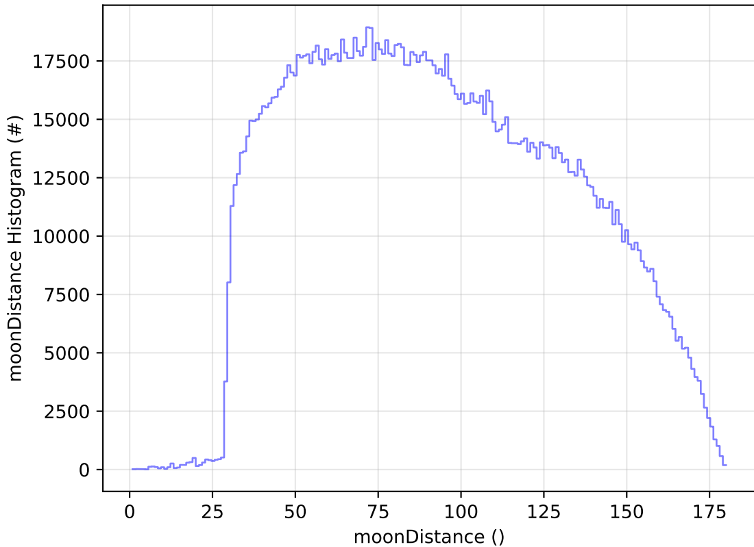
too_elab_r32_d3_griz_v3.4_10yrs WFD all bands: moonDistance Histogram
