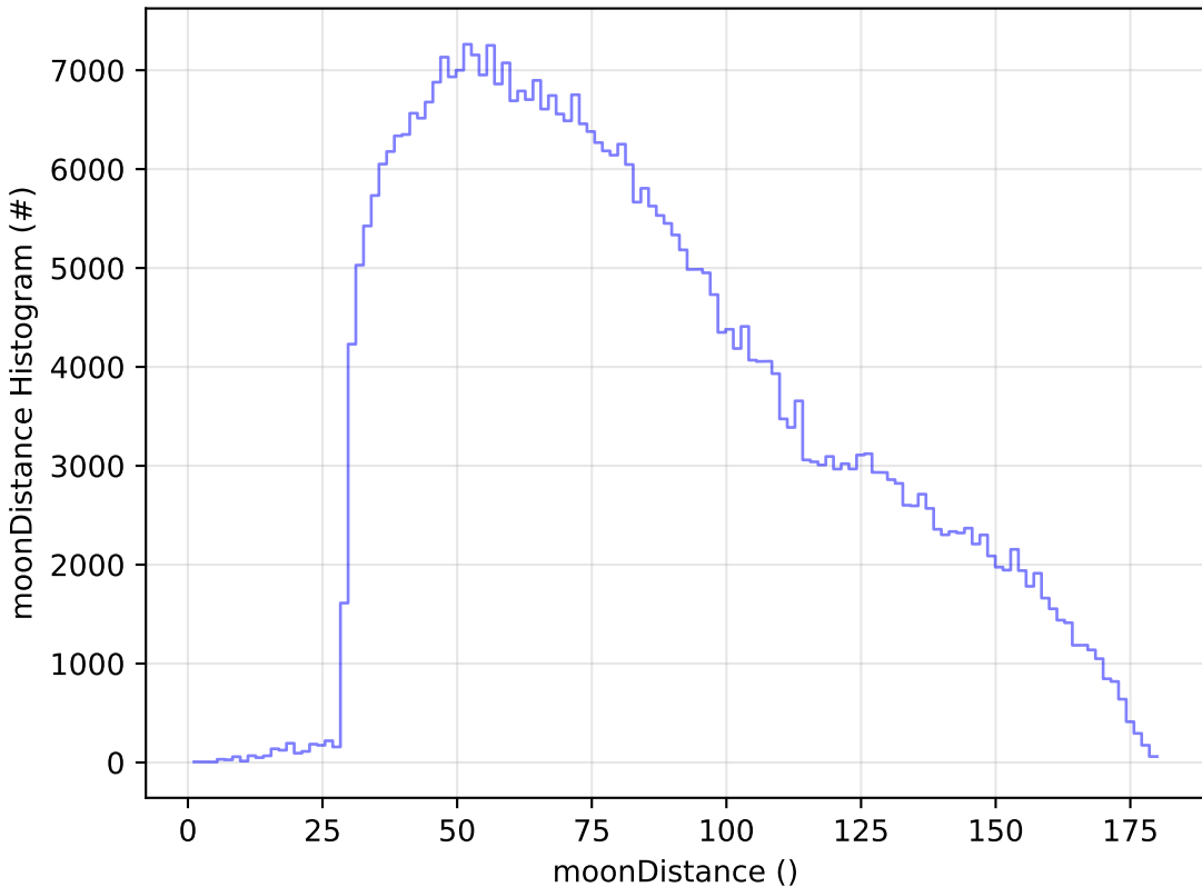
too_elab_r32_d3_griz_v3.4_10yrs All sky z band: moonDistance Histogram
