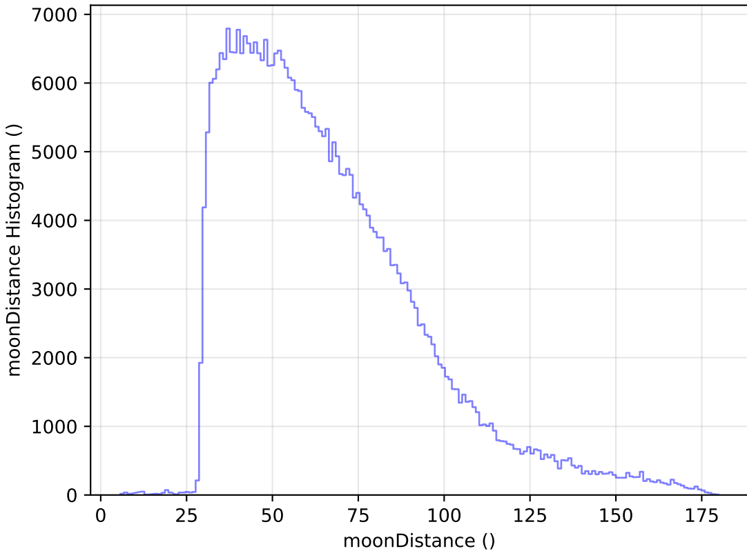
too_elab_r32_d3_griz_v3.4_10yrs All sky y band: moonDistance Histogram
