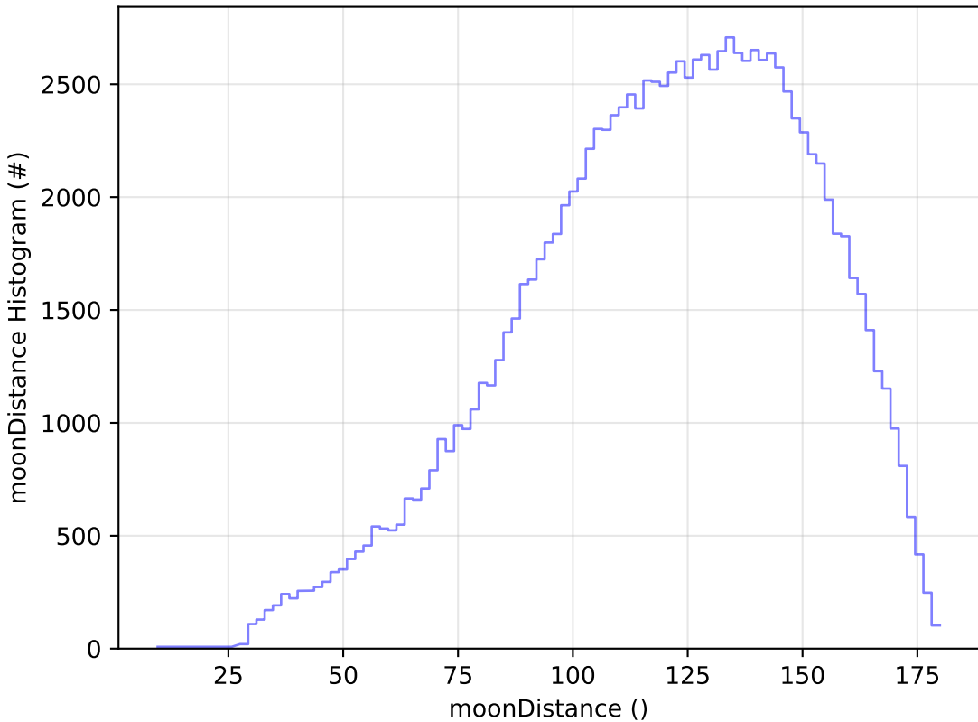
too_elab_r32_d3_griz_v3.4_10yrs All sky u band: moonDistance Histogram
