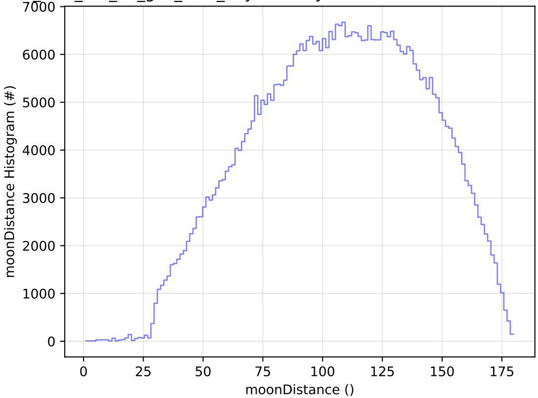
too_elab_r32_d3_griz_v3.4_10yrs All sky r band: moonDistance Histogram
