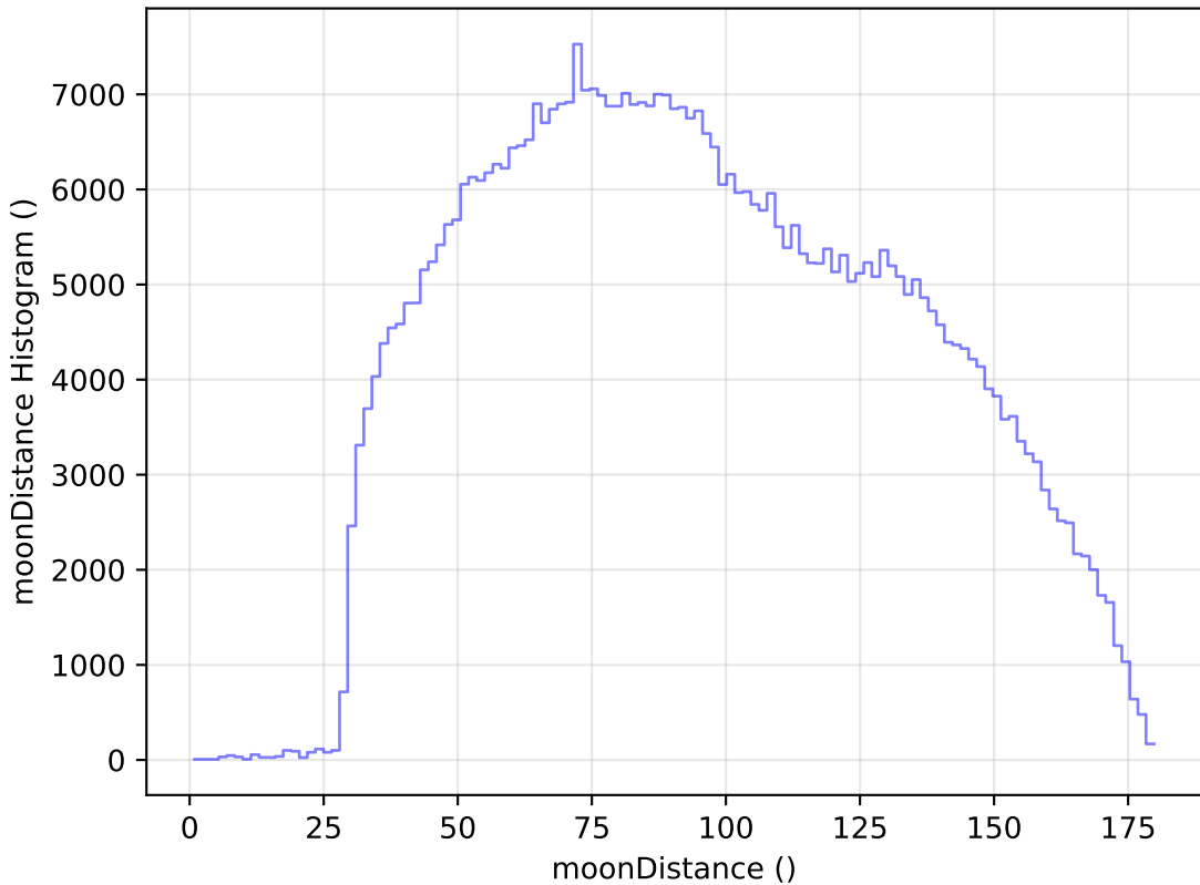
too_elab_r32_d3_griz_v3.4_10yrs All sky i band: moonDistance Histogram
