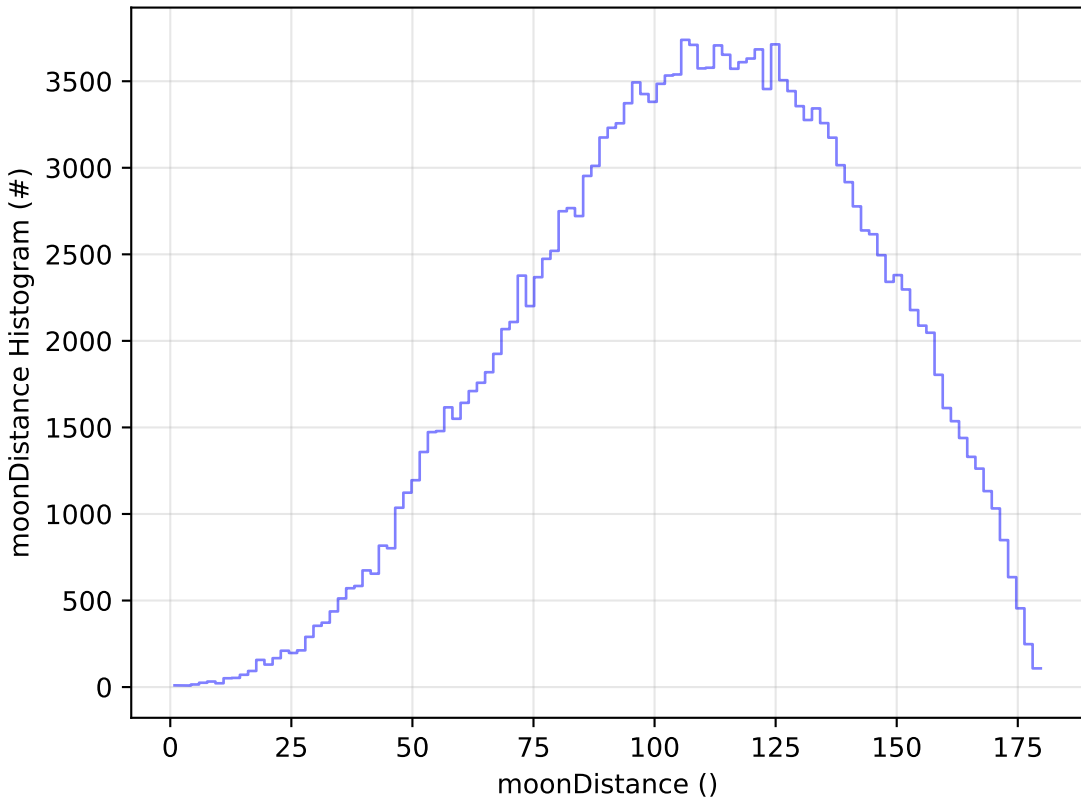
too_elab_r32_d3_griz_v3.4_10yrs All sky g band: moonDistance Histogram
