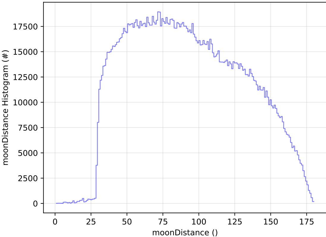
too_elab_r32_d3_griz_v3.4_10yrs All sky all bands: moonDistance Histogram
