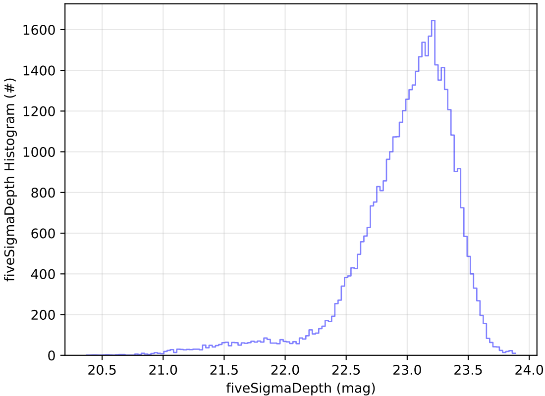
too_elab_r32_d3_griz_v3.4_10yrs Yr 1 z band: fiveSigmaDepth Histogram
