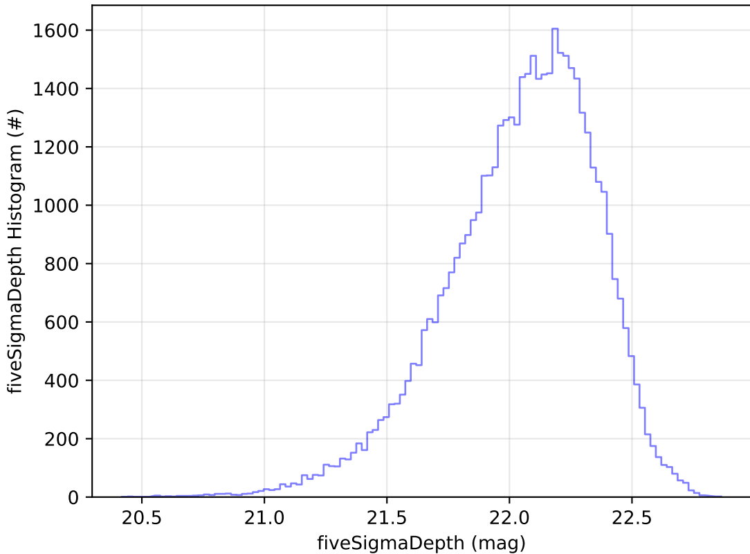
too_elab_r32_d3_griz_v3.4_10yrs Yr 1 y band: fiveSigmaDepth Histogram
