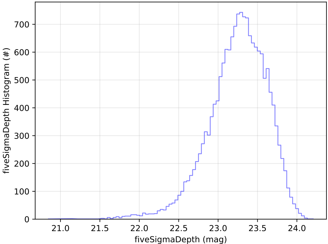
too_elab_r32_d3_griz_v3.4_10yrs Yr 1 u band: fiveSigmaDepth Histogram
