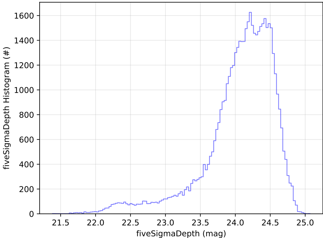
too_elab_r32_d3_griz_v3.4_10yrs Yr 1 r band: fiveSigmaDepth Histogram
