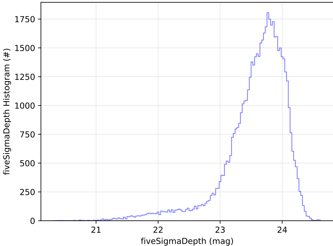
too_elab_r32_d3_griz_v3.4_10yrs Yr 1 i band: fiveSigmaDepth Histogram
