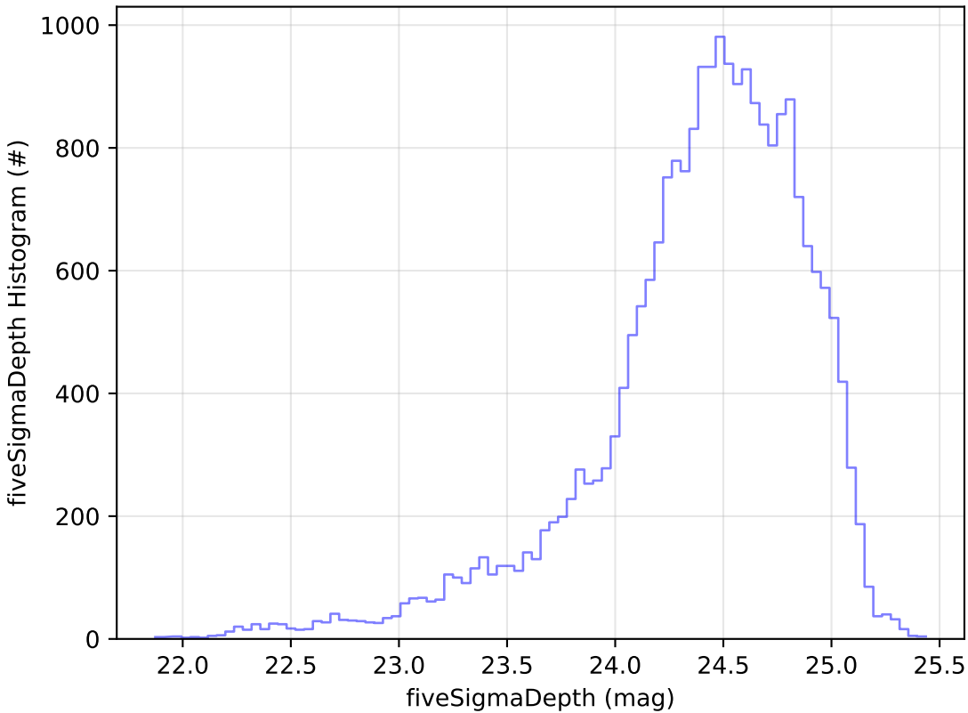
too_elab_r32_d3_griz_v3.4_10yrs Yr 1 g band: fiveSigmaDepth Histogram
