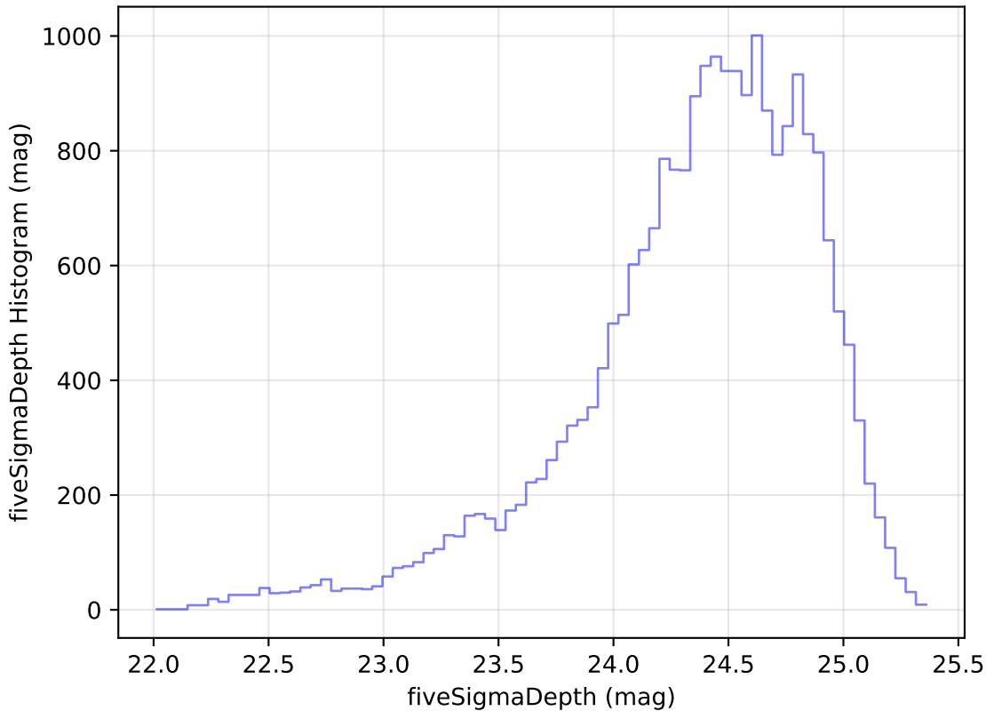
too_elab_r32_d3_griz_v3.4_10yrs Yr 1 g band: fiveSigmaDepth Histogram
