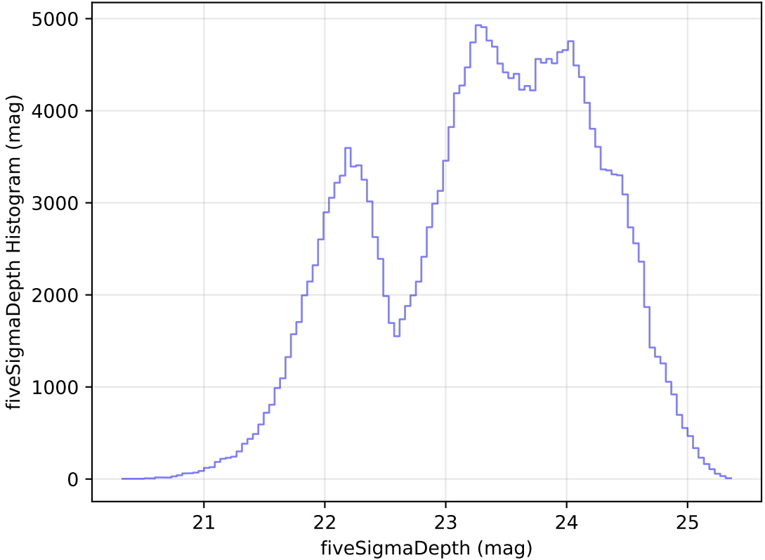
too_elab_r32_d3_griz_v3.4_10yrs Yr 1 all bands: fiveSigmaDepth Histogram
