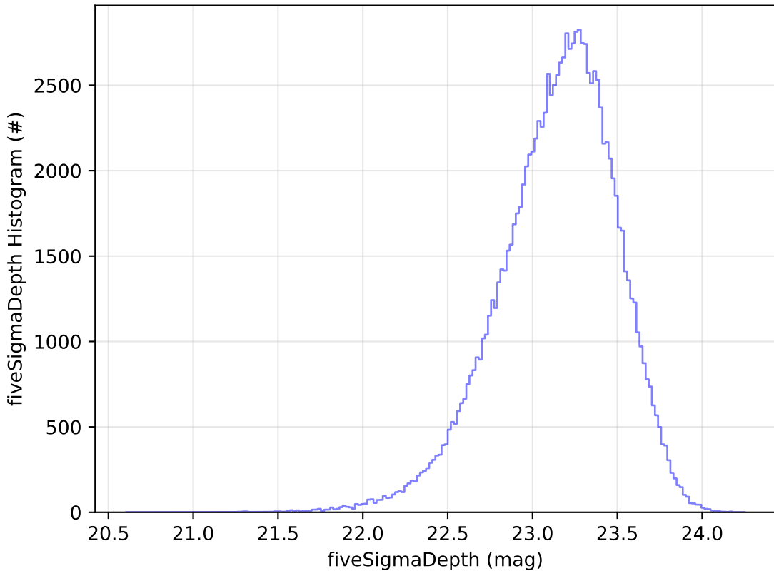
too_elab_r32_d3_griz_v3.4_10yrs WFD u band: fiveSigmaDepth Histogram
