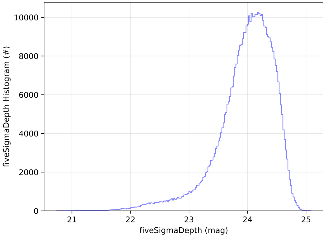
too_elab_r32_d3_griz_v3.4_10yrs WFD r band: fiveSigmaDepth Histogram
