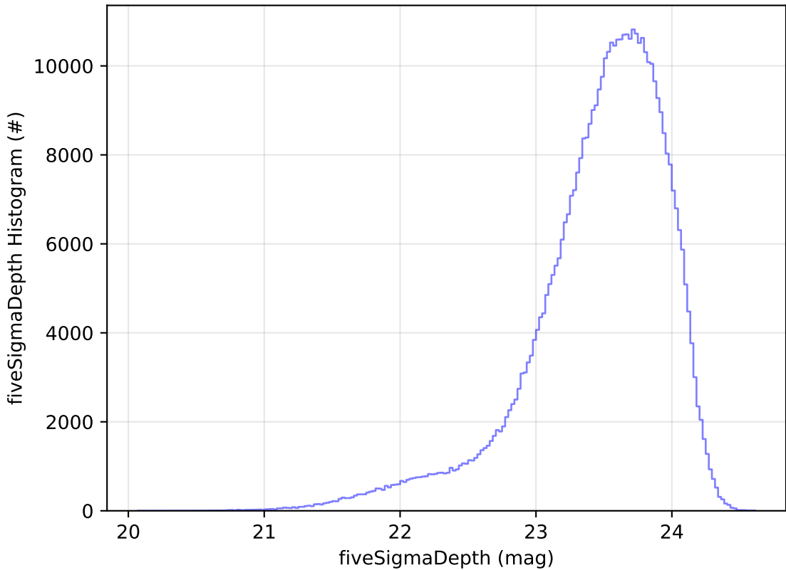
too_elab_r32_d3_griz_v3.4_10yrs WFD i band: fiveSigmaDepth Histogram
