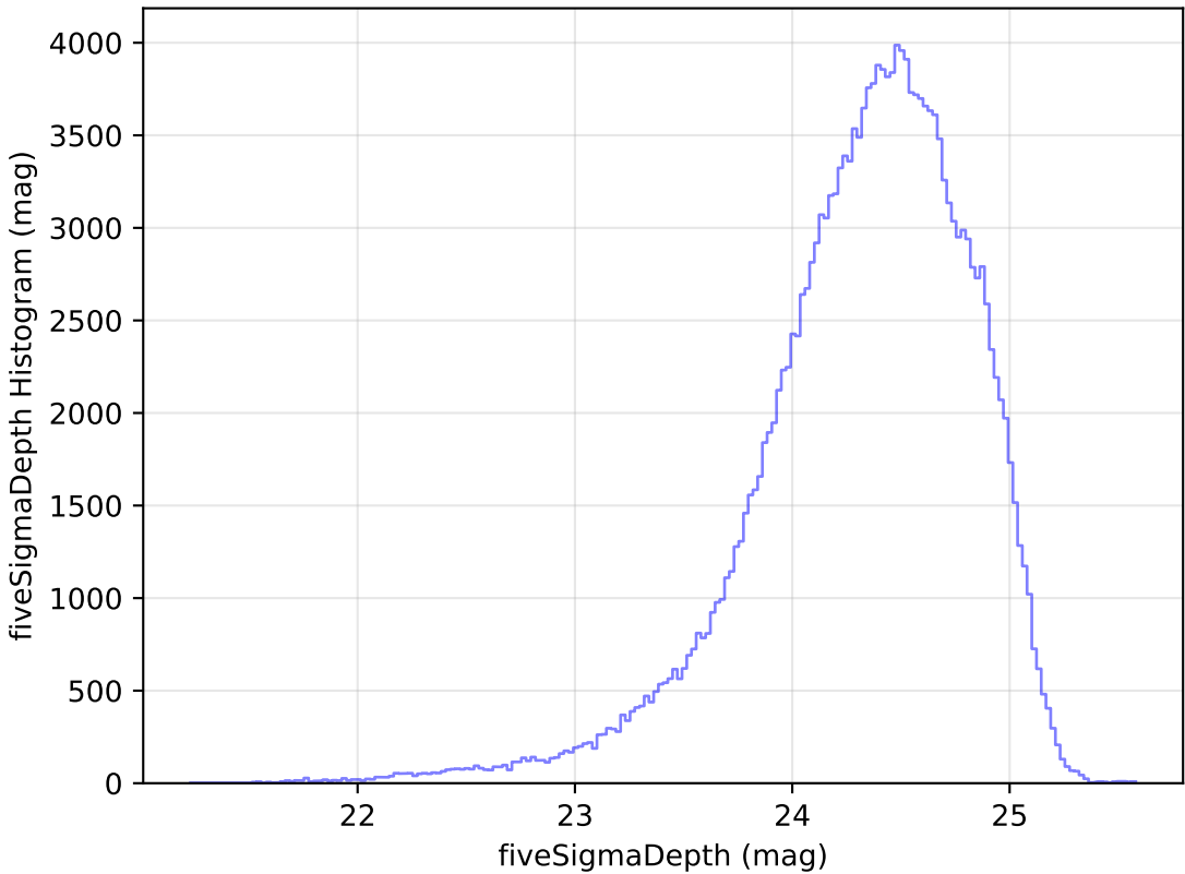
too_elab_r32_d3_griz_v3.4_10yrs WFD g band: fiveSigmaDepth Histogram
