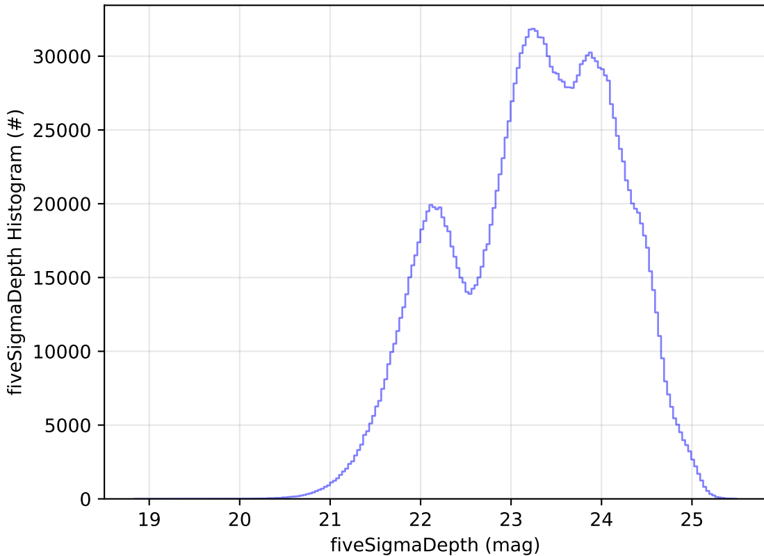
too_elab_r32_d3_griz_v3.4_10yrs WFD all bands: fiveSigmaDepth Histogram
