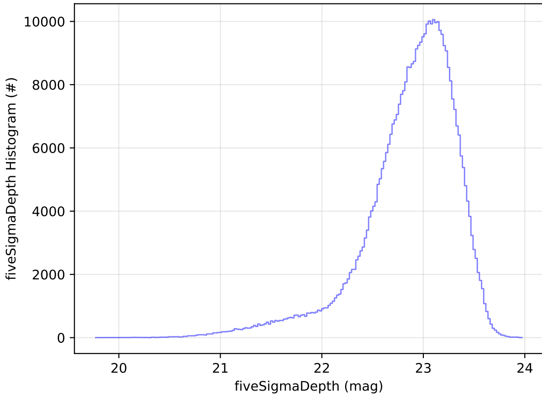
too_elab_r32_d3_griz_v3.4_10yrs All sky z band: fiveSigmaDepth Histogram
