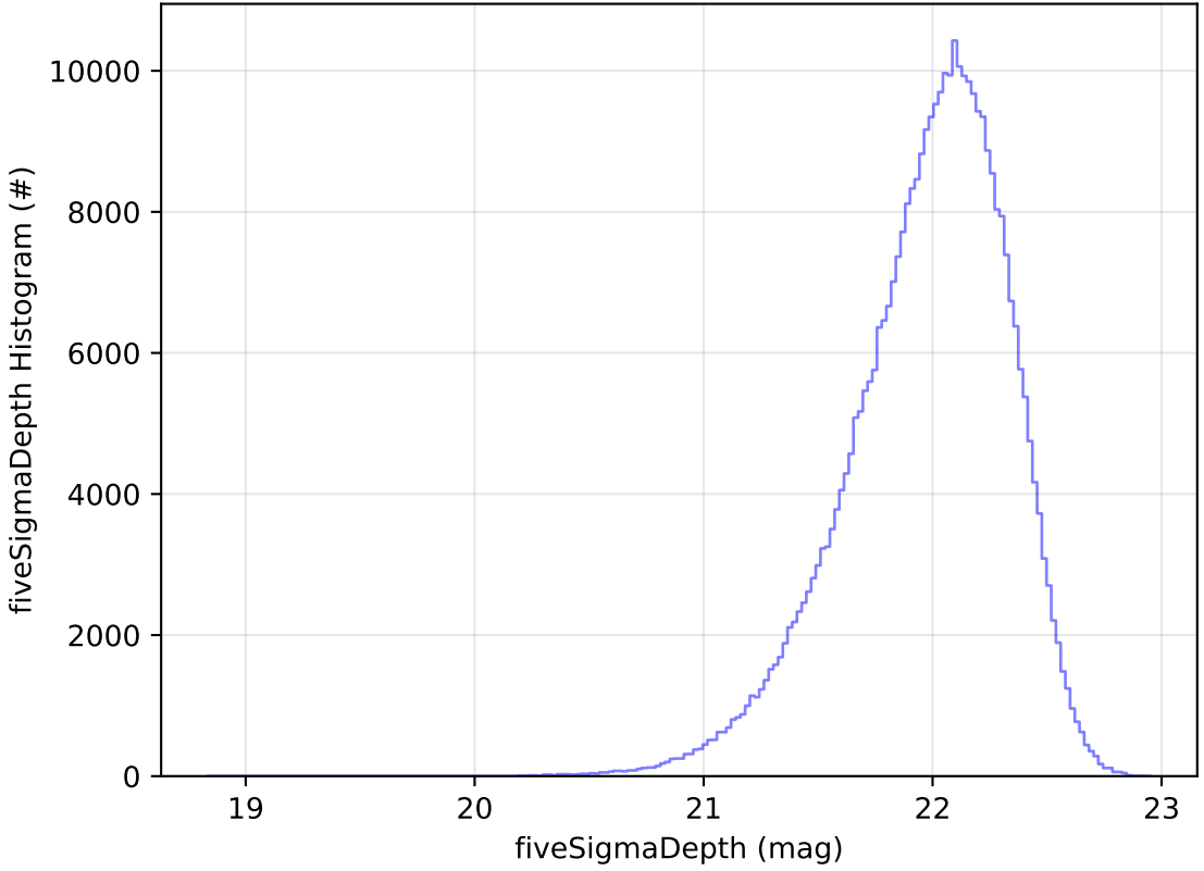
too_elab_r32_d3_griz_v3.4_10yrs All sky y band: fiveSigmaDepth Histogram
