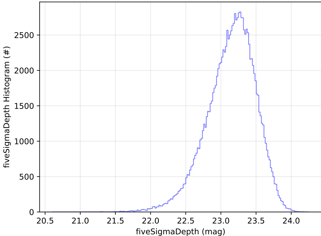
too_elab_r32_d3_griz_v3.4_10yrs All sky u band: fiveSigmaDepth Histogram
