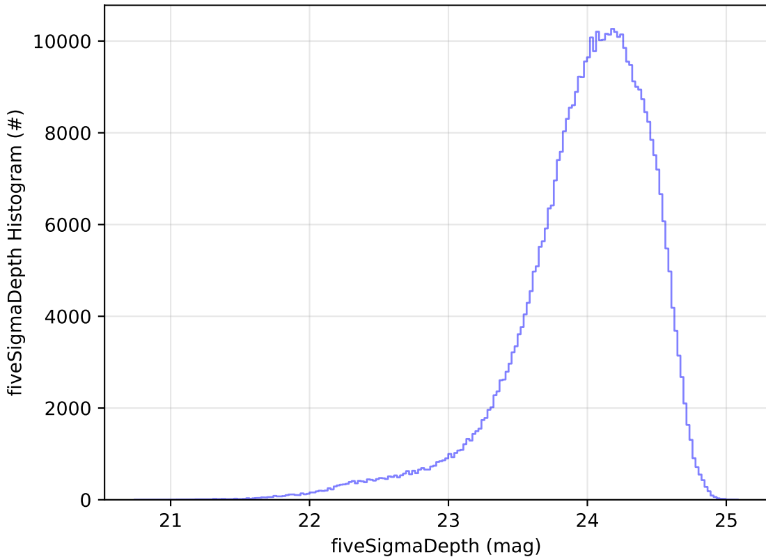
too_elab_r32_d3_griz_v3.4_10yrs All sky r band: fiveSigmaDepth Histogram
